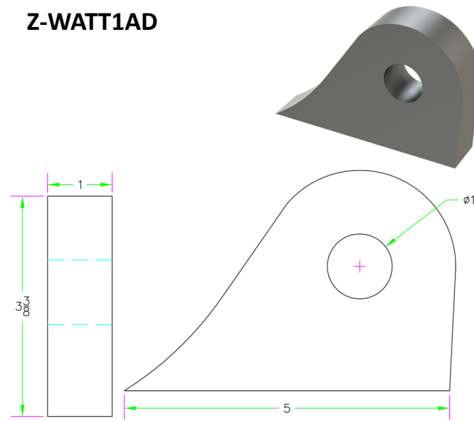
1" T1 - Replacement Ear for Watts Ripper Shank - Plain
