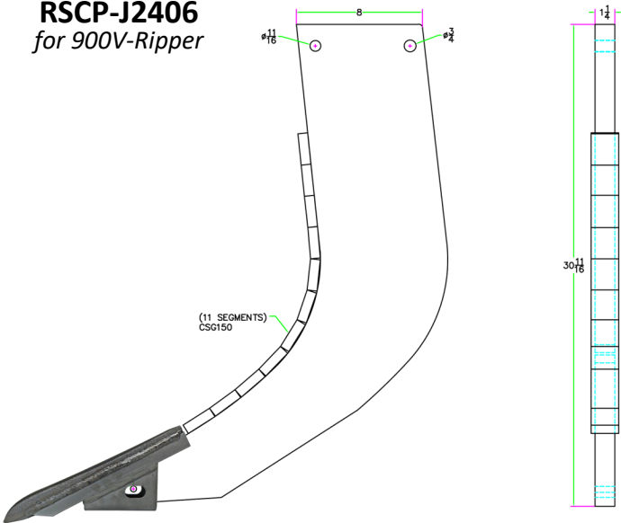
1-1/4" T1 Ripper Shank - with Chrome Shin Guard & RCHJ21507 Chrome Point
