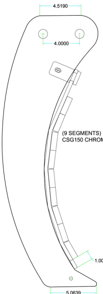
1" T1 Shank - w/Bolt-On Shin Guard
