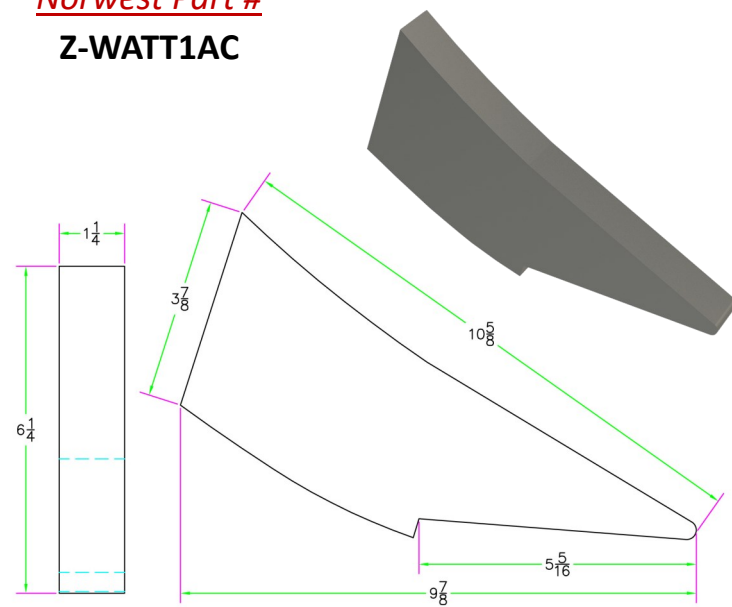
1-1/4" T1 - Replacement Tip for Watts Ripper Shank - Plain
