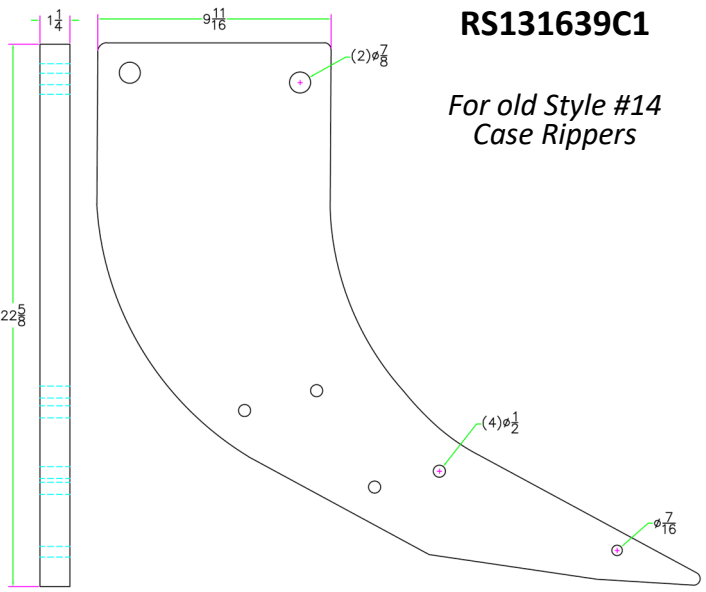
1-1/4" T1 Ripper Shank - Plain
