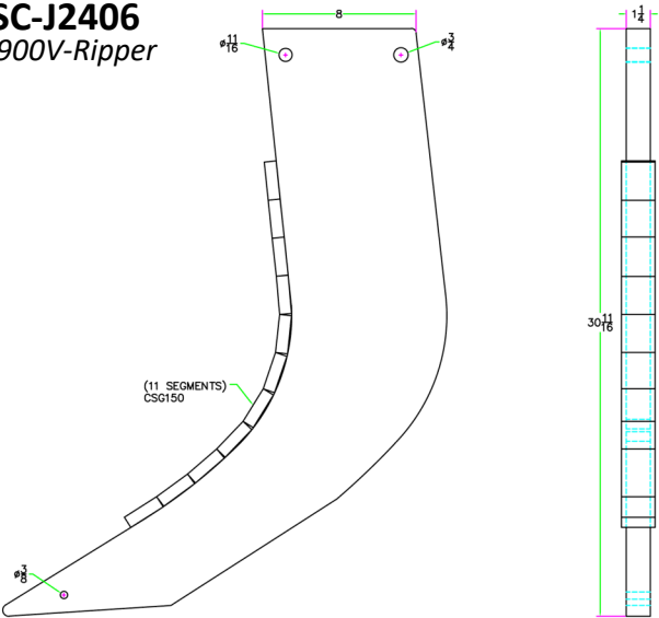
1-1/4" T1 Ripper Shank - with Chrome Shin Guard
