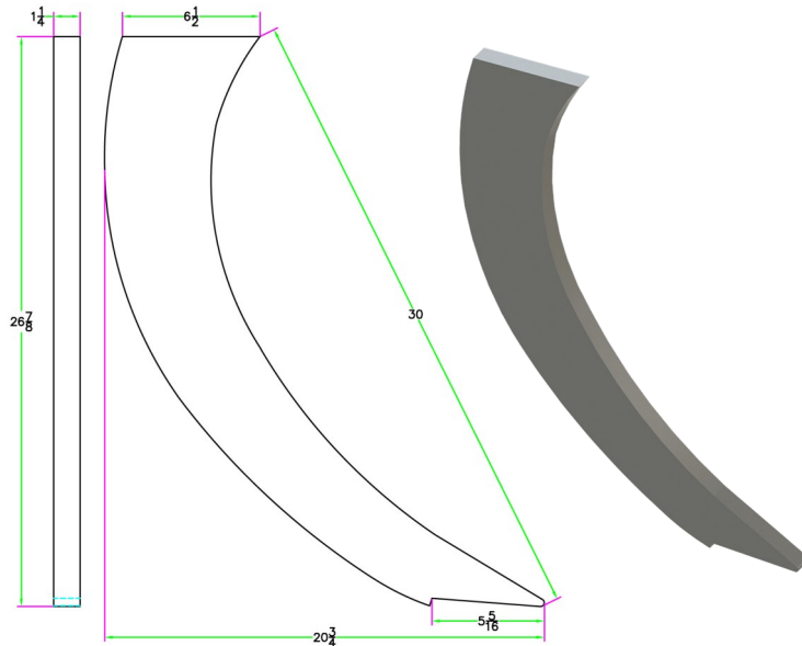
1-1/4" T1 - Replacement for Bottom Half of Watts Ripper Shank - Plain
