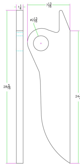
1-1/4" T1 - Replacement for Top Half of Watts Ripper Shank - Plain
