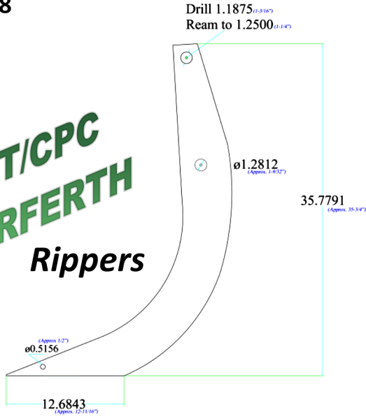
1-1/4" T1 Ripper Shank - Plain
