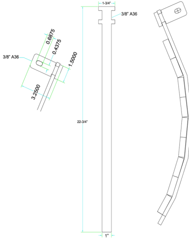
3/8" A36 Bolt-On Shin Guard w/ 7/16" x 11/16" Bolt Slot & 1-1/2" Chrome Segments
