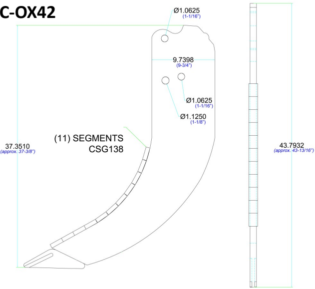
1" T1 Ripper Shank - with Chrome Shin Guard
