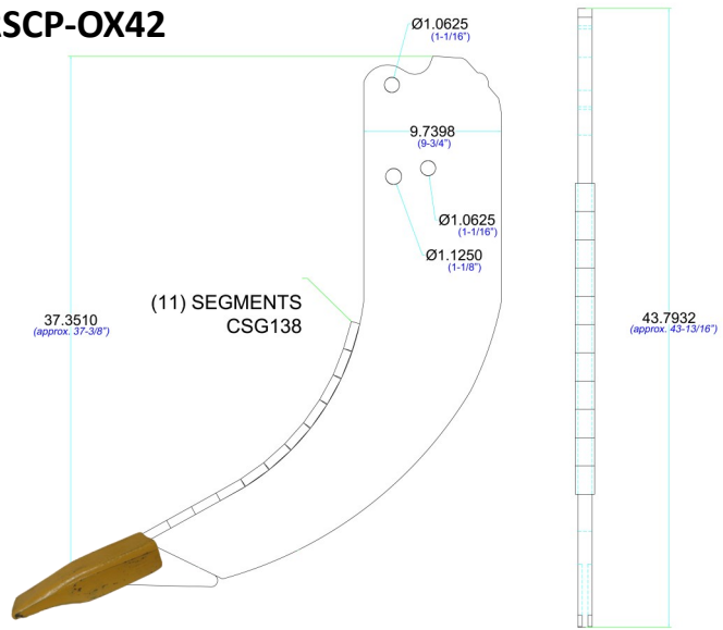
1" T1 Ripper Shank - with Chrome Shin Guard & RP2D-5 Plain Drop Forged Point
