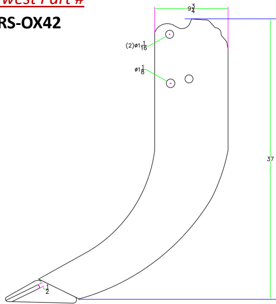
1" T1 Ripper Shank - Plain
