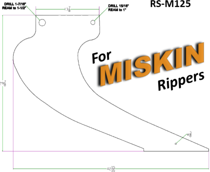
1-1/4" T1 or Plow Steel Ripper Shank - Plain
